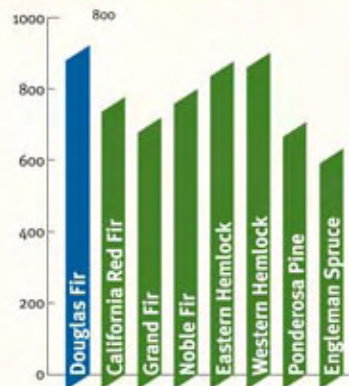
SHEARING STRENGTH (PARALLEL TO GRAIN)
