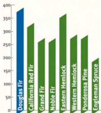
CRUSHING STRENGTH (PERPENDICULAR TO GRAIN)
