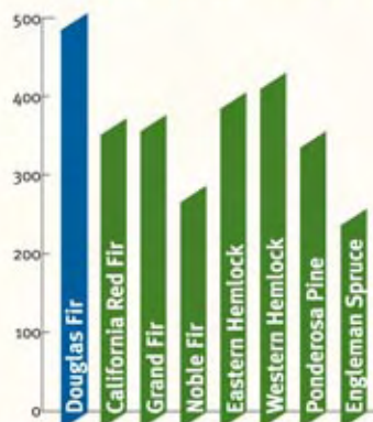
SIDE HARDNESS (PERPENDICULAR TO GRAIN)
