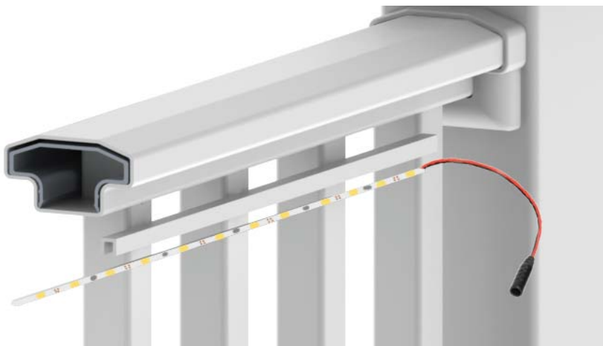
Under Rail Light Channel (92" length) shown with Under-Rail Lighting (92" length - 3W)
